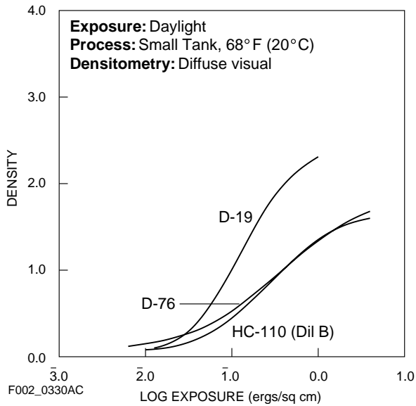
Characteristic Curves for KODAK High Speed Infrared Film / HIE
