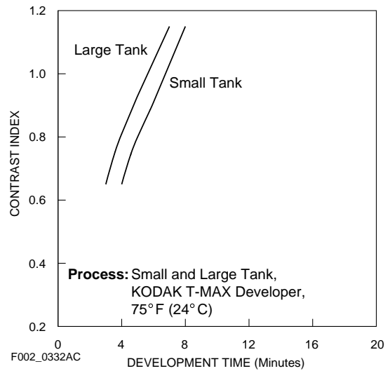
Contrast-Index Curves for KODAK High Speed Infrared Film / HIE
